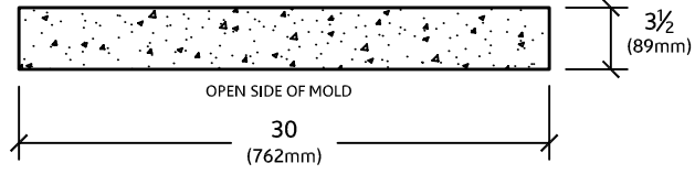
ELEVATION VIEW
