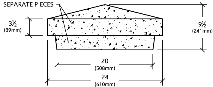
ELEVATION VIEW
