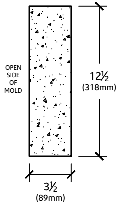
SECTION VIEW
