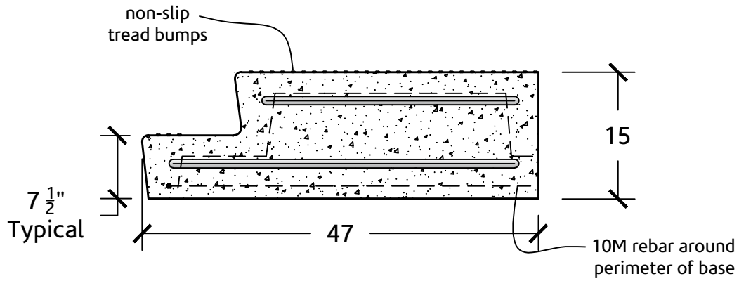
ELEVATION VIEW
