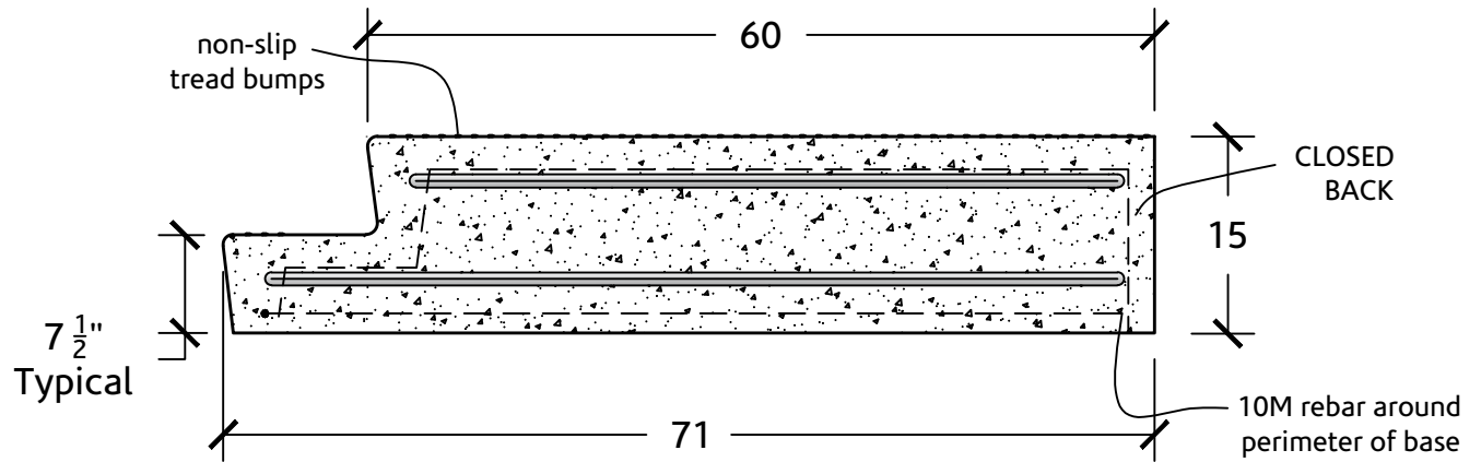
ELEVATION VIEW
