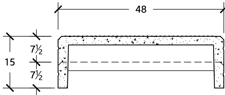
SECTION VIEW
