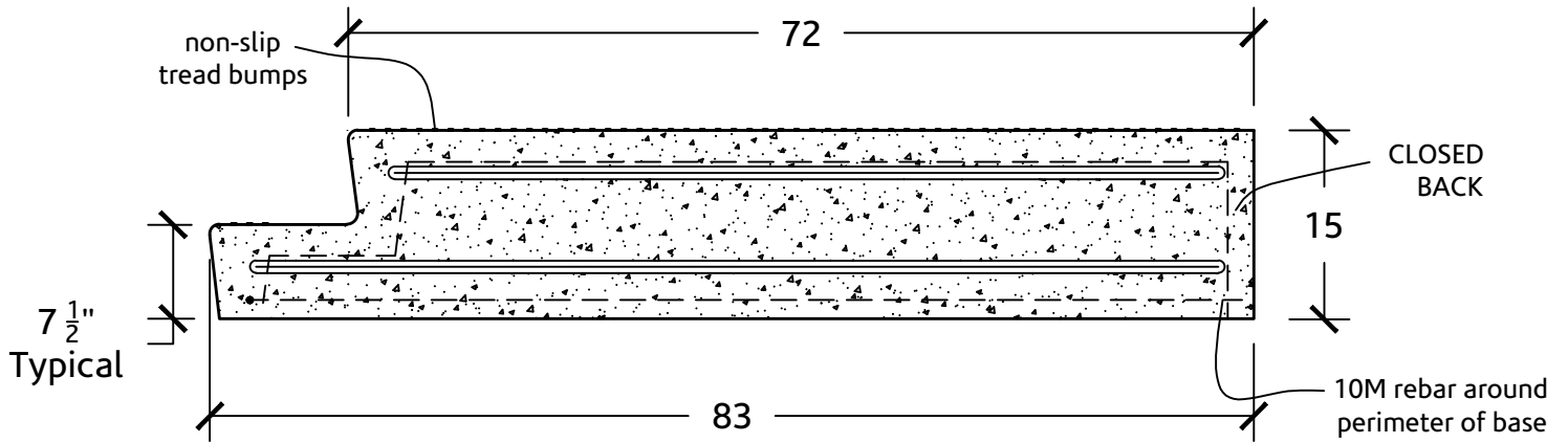
ELEVATION VIEW
