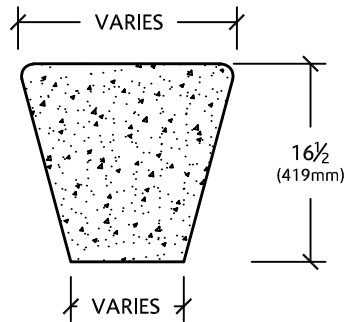
SECTION VIEW
