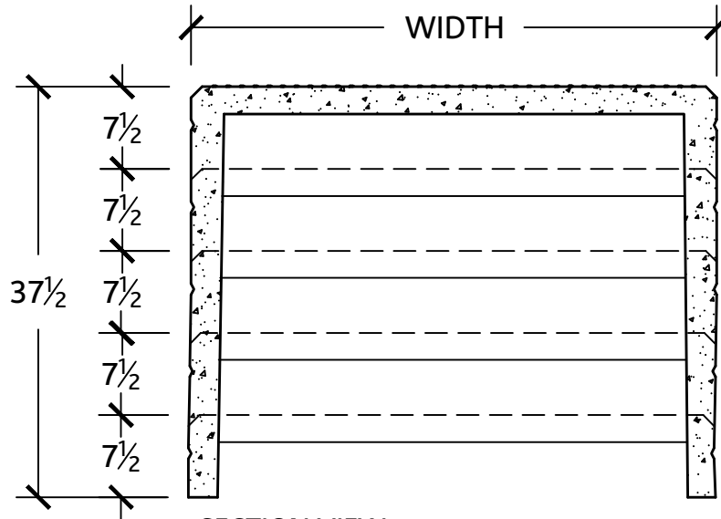
SECTION VIEW
