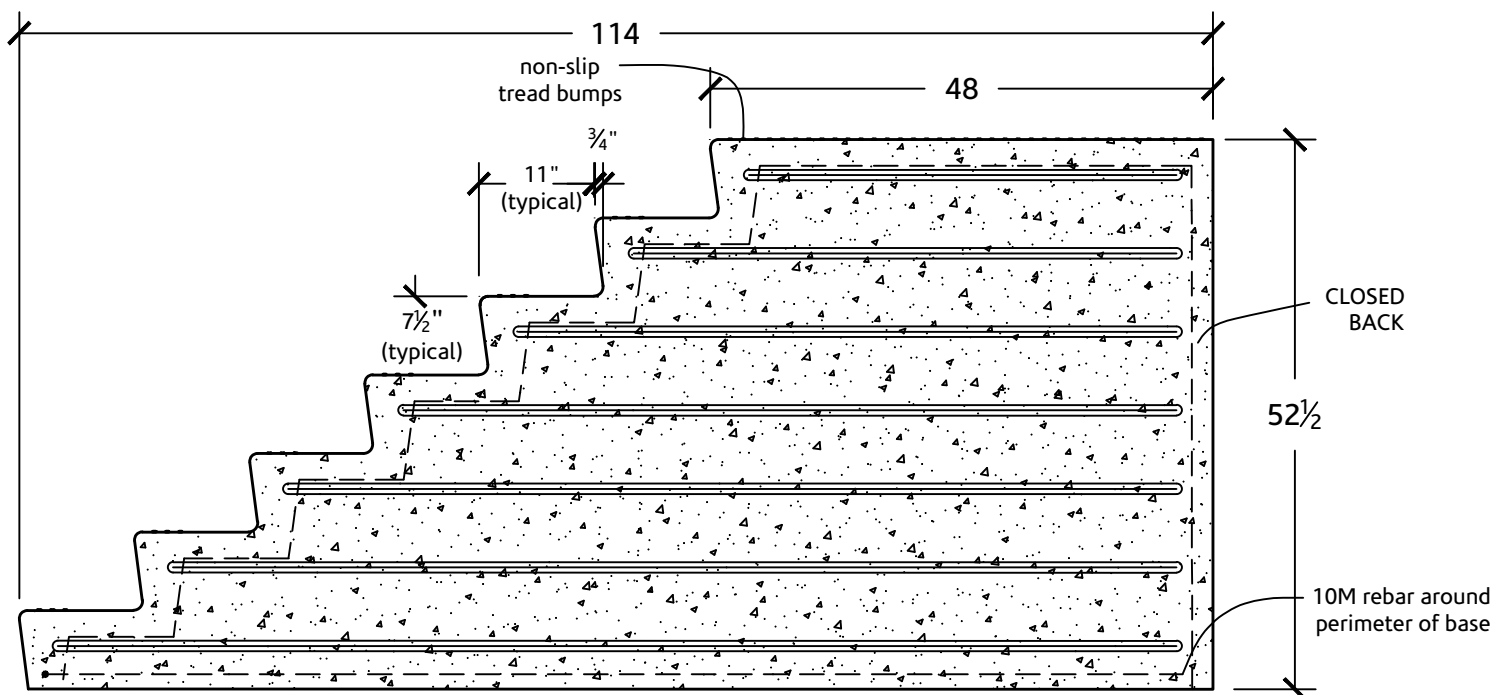
ELEVATION VIEW
