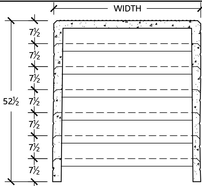
SECTION VIEW
