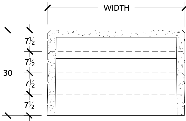
SECTION VIEW
