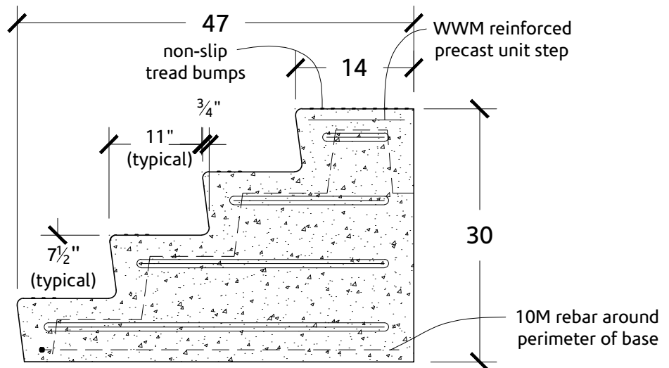
ELEVATION VIEW
