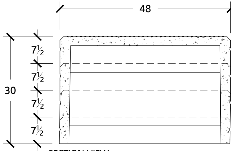
SECTION VIEW
