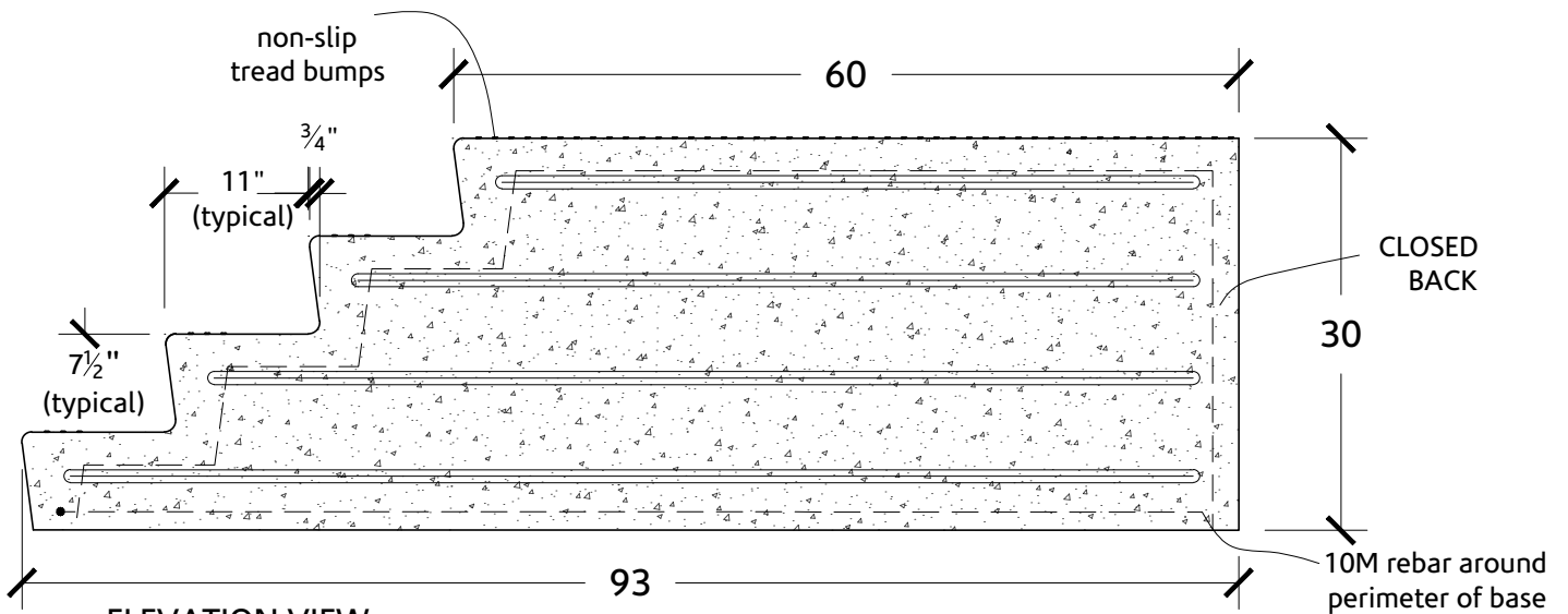
ELEVATION VIEW
