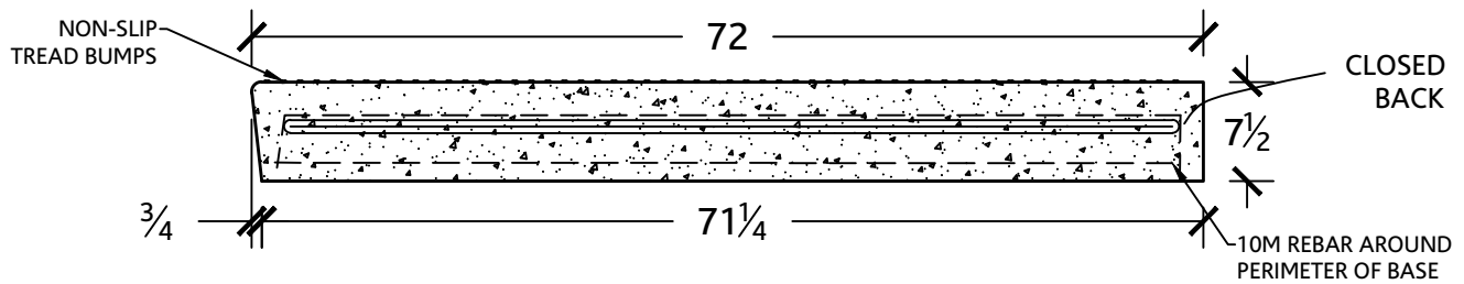
ELEVATION VIEW
