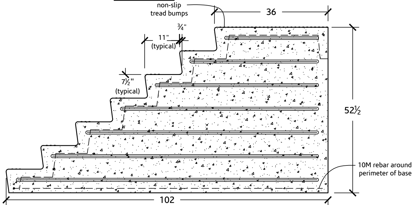
ELEVATION VIEW
