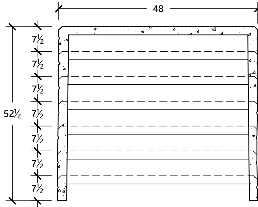
SECTION VIEW
