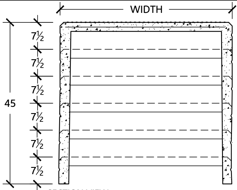
SECTION VIEW
