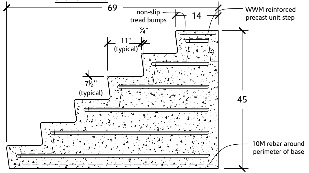
ELEVATION VIEW
